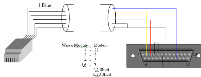
RJ 45 (to Wisco Module) ↔ DB 25 male (to Modem)
